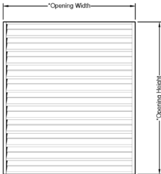
FRONT ELEVATION
