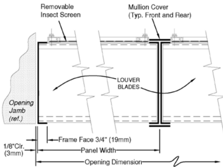
TYPICAL HORIZONTAL SECTION
